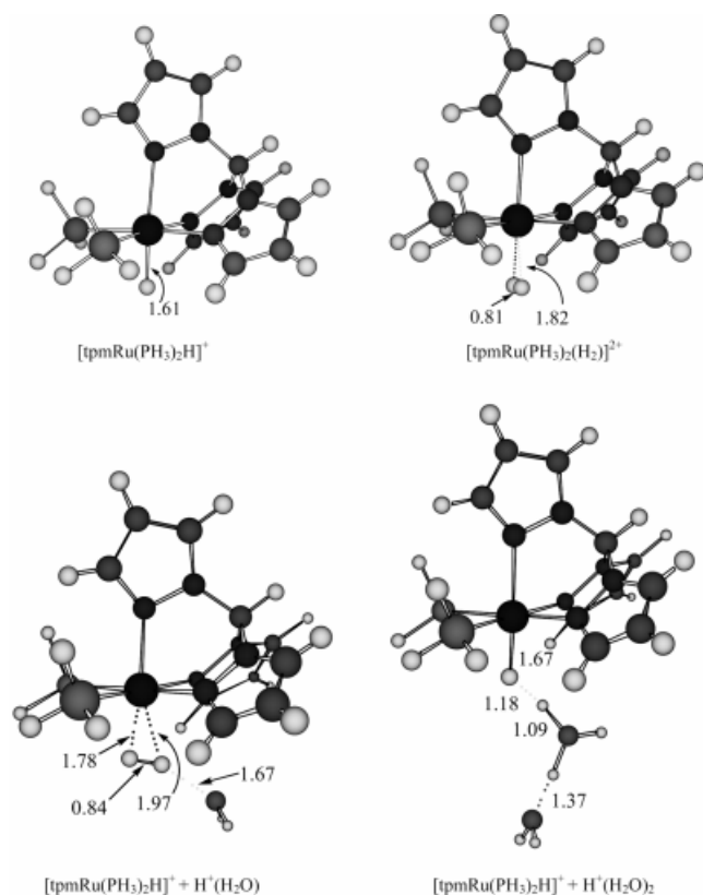
Figure 2. Optimized structures for model systems: [\text{tpmRu}(\text{PH}_3)_2\text{H}]^+ , [\text{tpmRu}(\text{PH}_3)_2(\eta^2\text{-H}_2)]^{2+} , [\text{tpmRu}(\text{PH}_3)_2\text{H}]^+ + \text{H}^+(\text{H}_2\text{O}) , and [\text{tpmRu}(\text{PH}_3)_2\text{H}]^+ + \text{H}^+(\text{H}_2\text{O})_2 .
