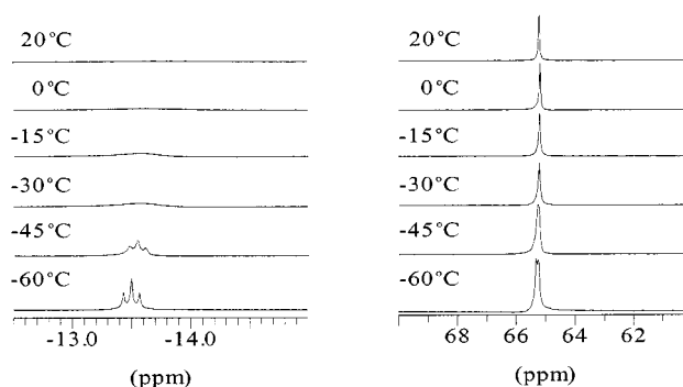
Figure 1. Variable-temperature (left) 1 H-NMR spectra (upfield region) and (right) 31 P-NMR spectra of [tpmRu(PPh 3 ) 2 H] + + aq HBF 4 in [D 8 ]THF
